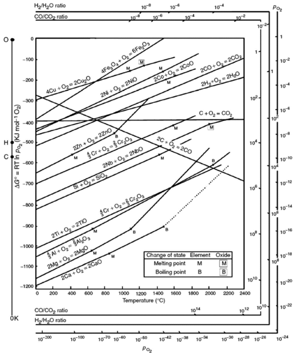
Figure 1: Ellingham diagram
