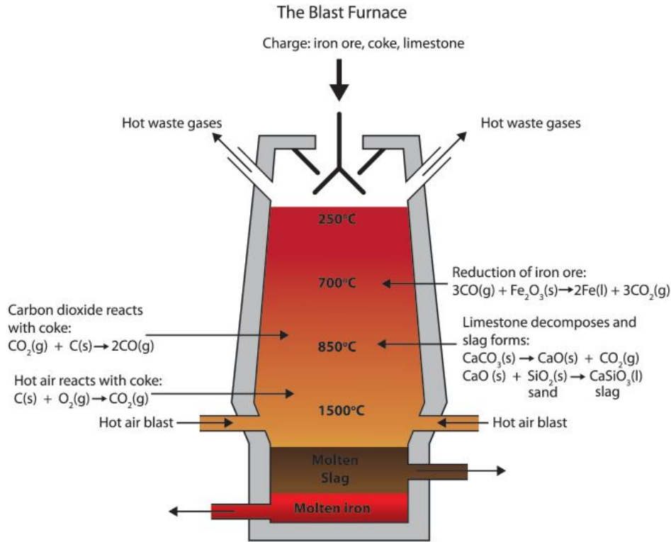
Figure 2: Blast furnace
